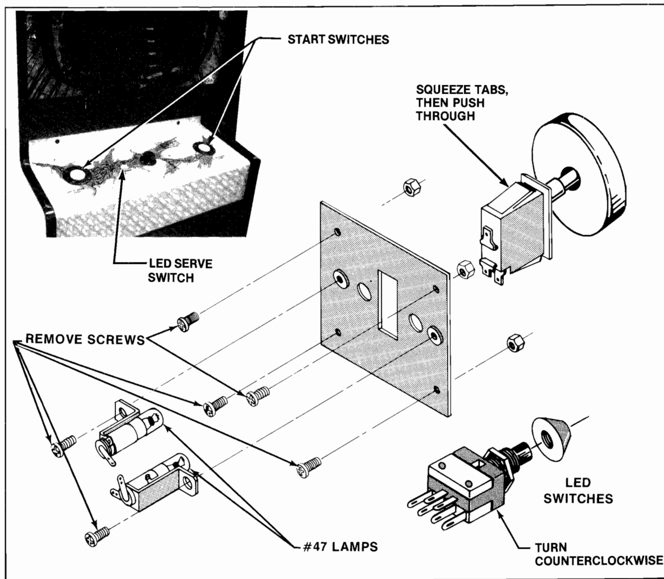
Figure 3-11 LICON and Button Switch Replacement
